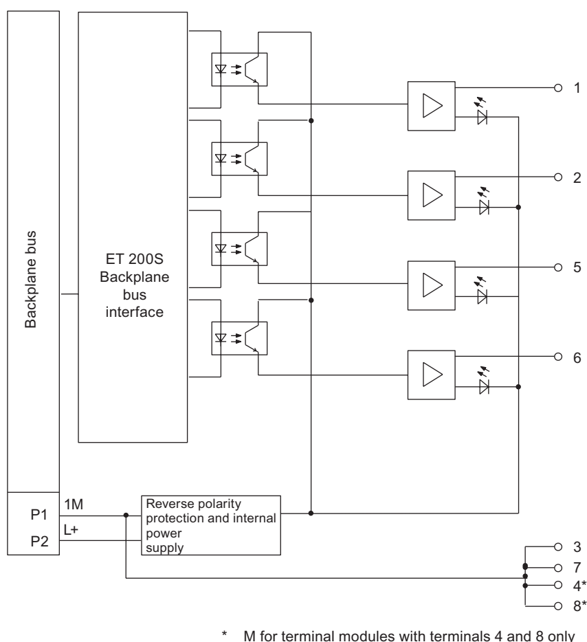
Figure 2-1 Block diagram of the 4DO DC24V/0.5A ST
